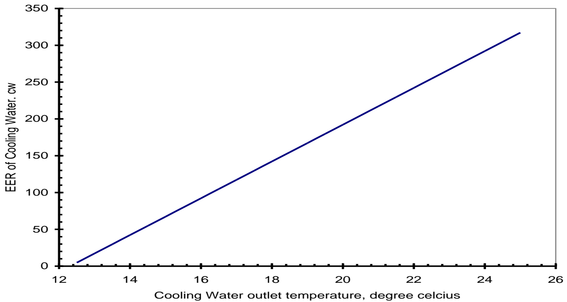
Fig. 4. Plot of EER of Cooling Water against Cooling Water outlet temperature. Figures 5 and 6 illustrate the influence of outlet cooling tower temperature on the COP and EER of cooling tower. The findings show that cooling tower performance is proportional to the temperature at the cooling tower outlet.
