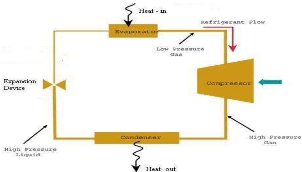
Fig. 1. Schematic illustration of the water chiller system's functioning concept. The operating parameters of the AC system, such as the temperature of the LSBLG 1200/MCF model chiller, the temperature of the cooling tower, and the temperature of the lubricating oil, were recorded for 8 hours at one-hour intervals using the in-built data display unit. The AC
