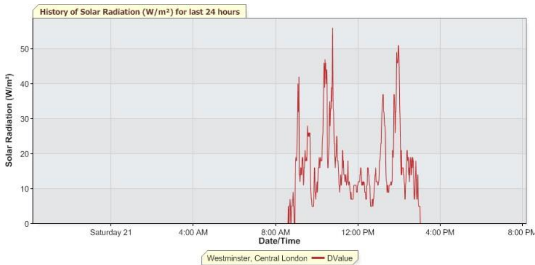
Fig. 4: Solar radiation for day-time with cloud impact
