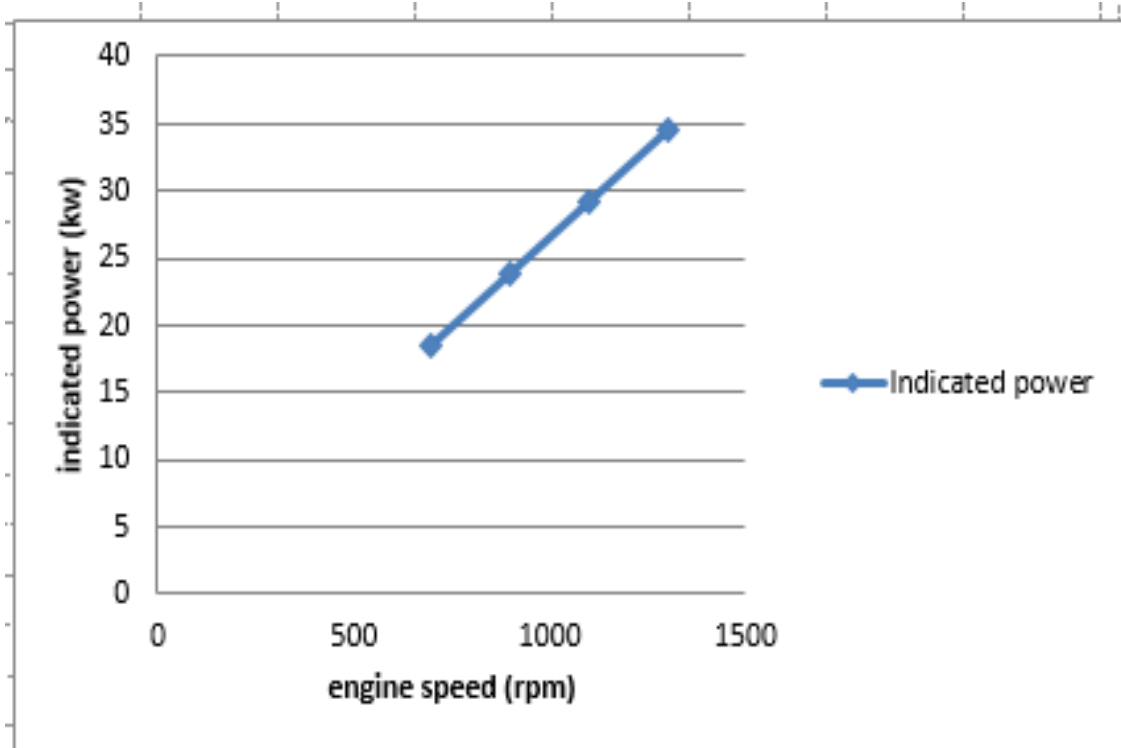
Fig 5. Indicated power versus engine speed
