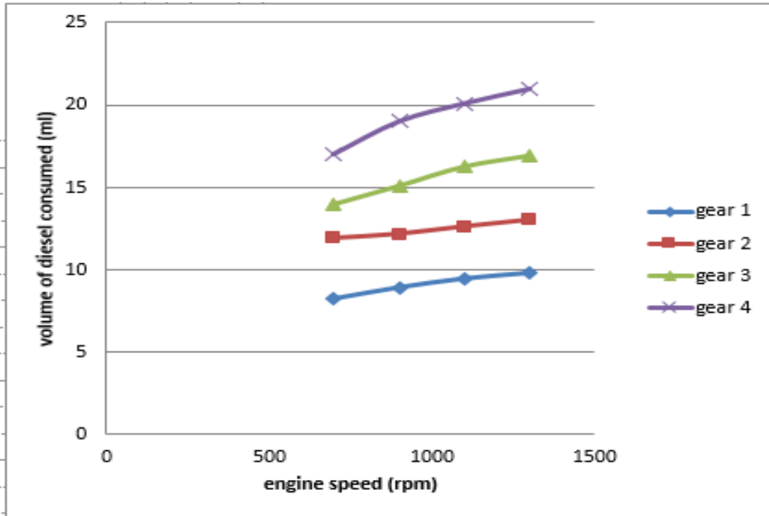
Fig.2. volume of diesel consumed versus engine speed
