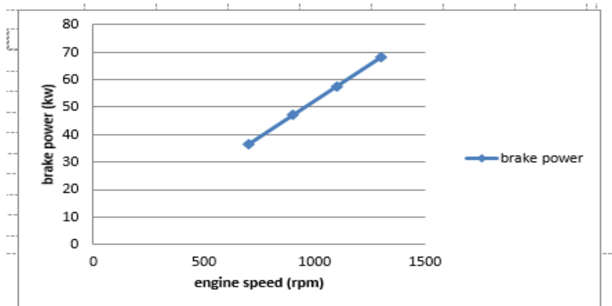
Fig 6. Brake power versus engine speed
