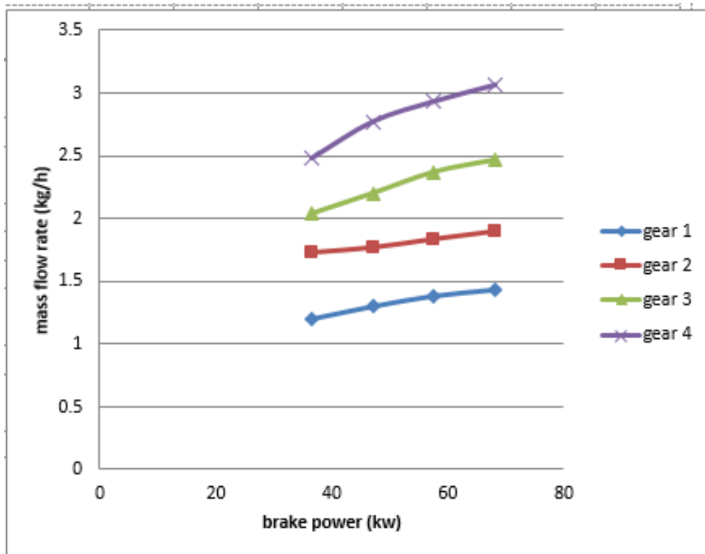
Fig 3. Mass flow rate versus brake power
