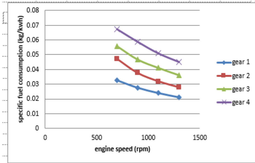
Fig 4 specific fuel consumption versus engine speed
